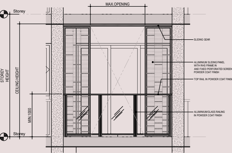
Typical Elevation (Open Position)
