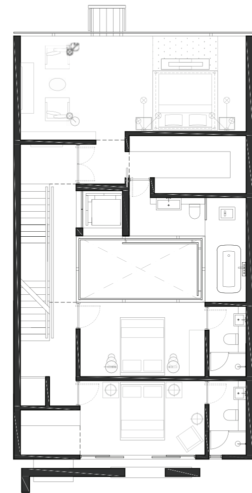
2ND FLOOR
