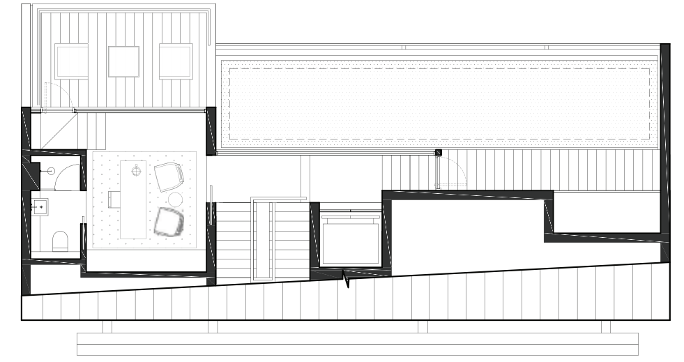
ATTIC
