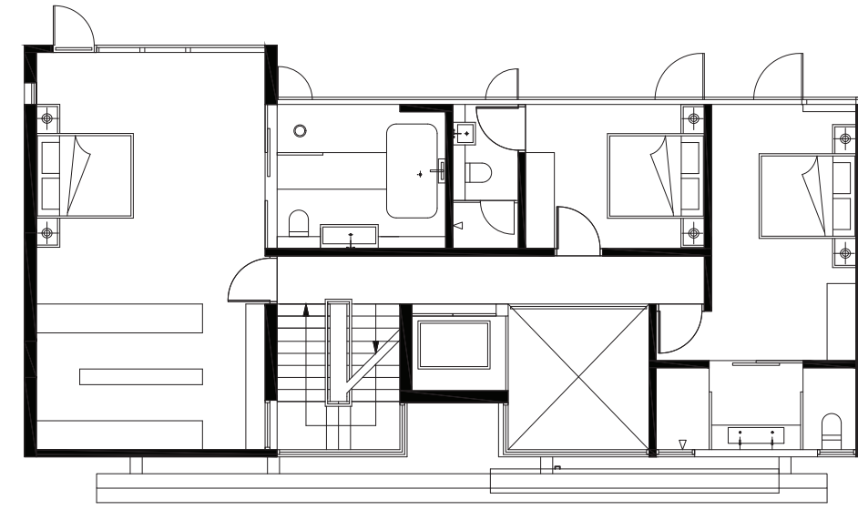
2ND FLOOR
