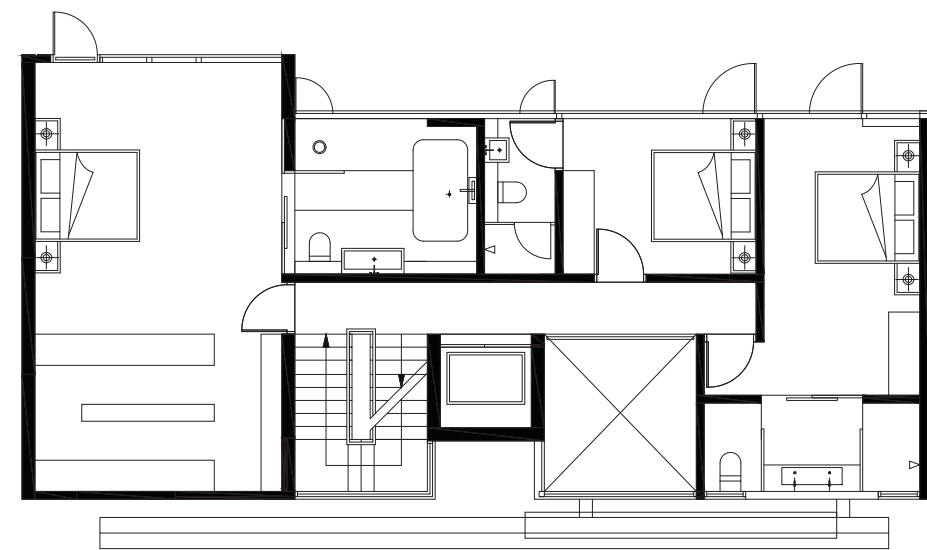
2ND FLOOR
