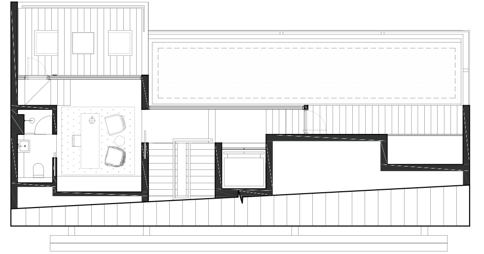
ATTIC
