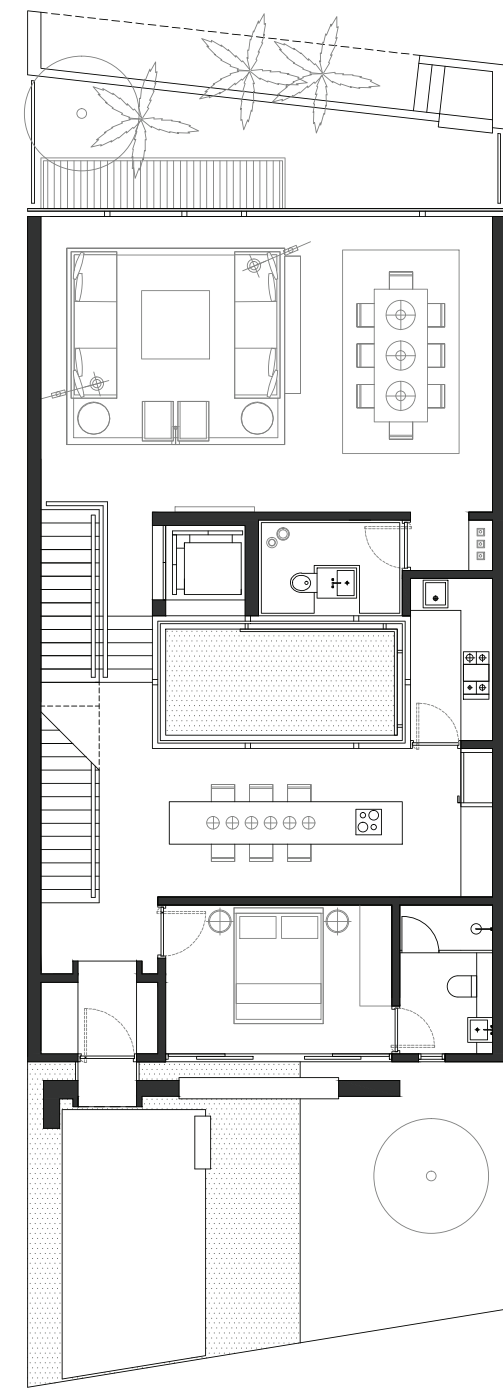
1ST FLOOR
