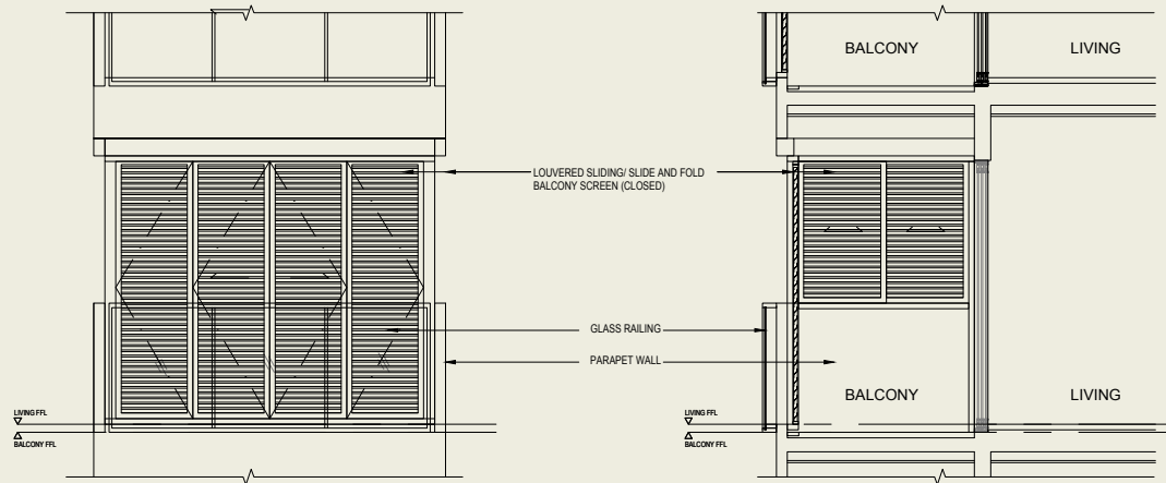
ELEVATION 1 (FRONT)
