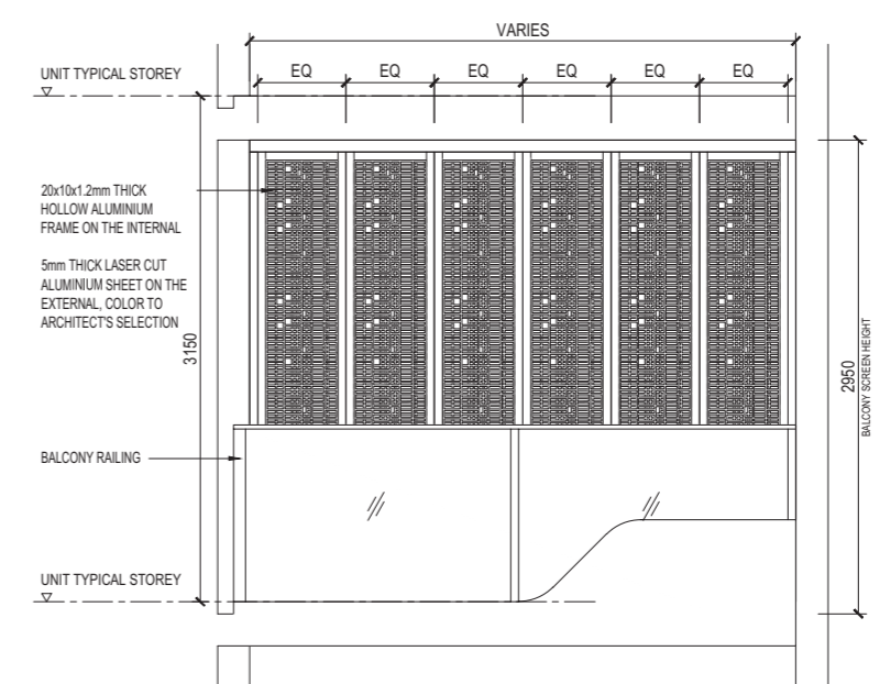
BALCONY SCREEN - FRONT ELEVATION (External View)
