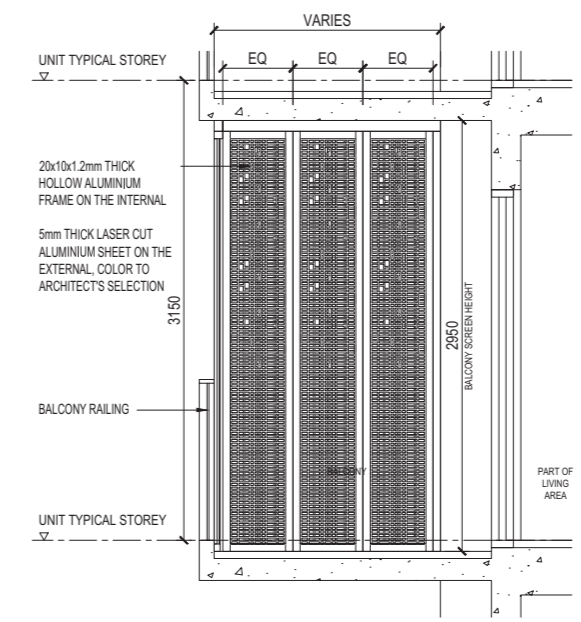
BALCONY SCREEN - SECTION A-A (Internal View)
