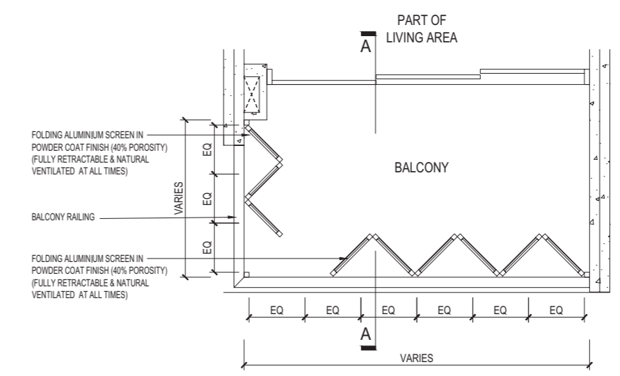
BALCONY SCREEN - PLAN
